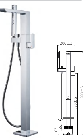
LD003 暗装落地浴缸龙头（铬色） Concealed floor-to-ceiling bathtub mixer (Chrome) (可定制明装)
