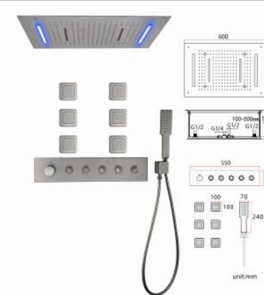
11AH5S243LJ4-Q 5 功能 LED 恒温套装（枪灰） Five-features LED thermostatic set (Gunmetal)
