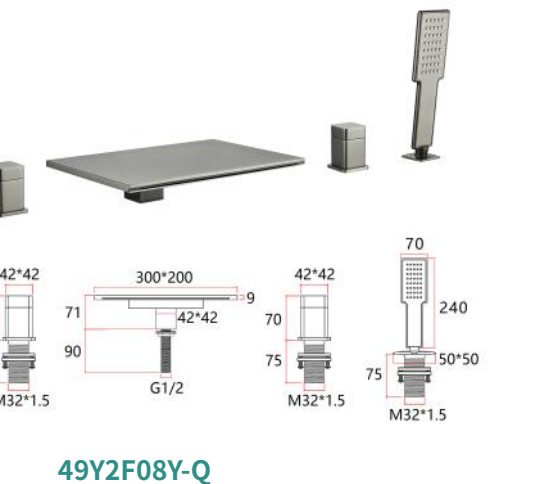
49Y2F08Y-Q 2 功能调温浴缸龙头（枪灰） Two-Function thermoregulation bathtub tap (Gunmetal) 浴缸瀑布、手持 Bathtub waterfall, hand held
