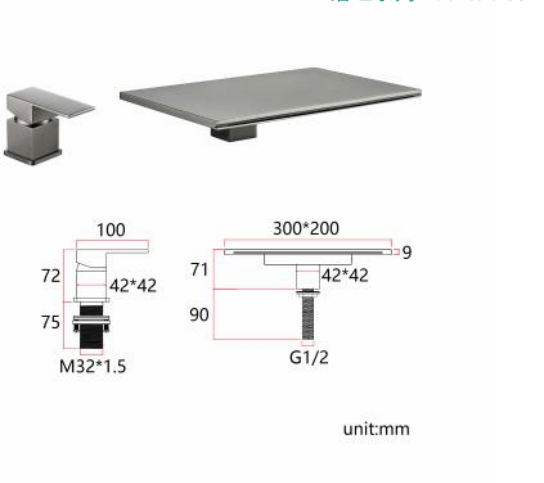
50Y1F08Y-Q 单功能调温浴缸龙头（枪灰） One-Function thermoregulation bathtub tap (Gold) 面盆瀑布 Basin waterfall
