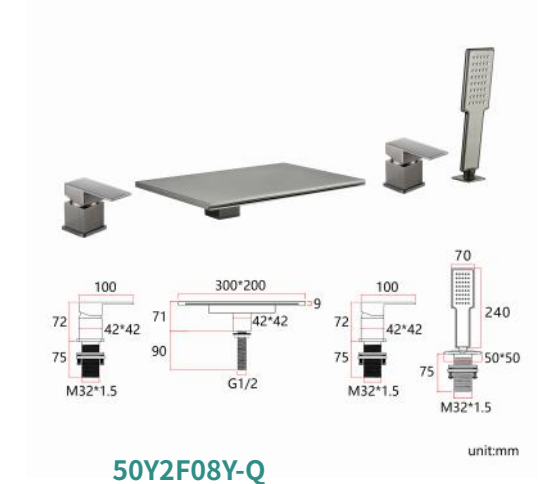
50Y2F08Y-Q 2 功能调温浴缸龙头（枪灰） Two-Function thermoregulation bathtub tap (Gunmetal) 浴缸瀑布、手持 Bathtub waterfall, hand held
