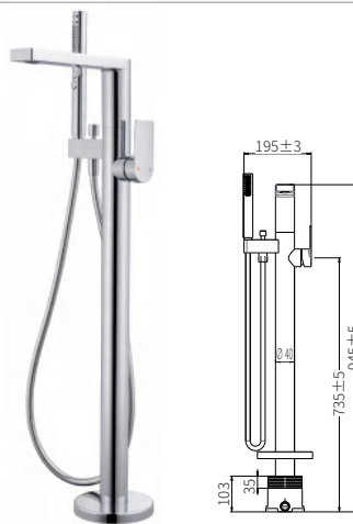
LD004 暗装落地浴缸龙头（铬色） Concealed floor-to-ceiling bathtub mixer (Chrome) (可定制明装)
