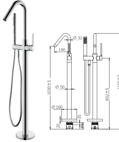
LDR002 暗装落地浴缸龙头（铬色） Concealed floor-to-ceiling bathtub mixer (Chrome) (可定制明装)
