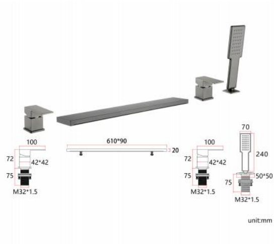
50Y2F24Y-Q 2 功能调温浴缸龙头（枪灰） Two-Function thermoregulation bathtub tap (Gunmetal) 浴缸瀑布、手持 Bathtub waterfall, hand held
